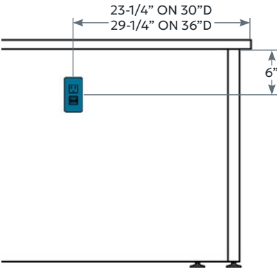
Carver Power on U-Shape Table
