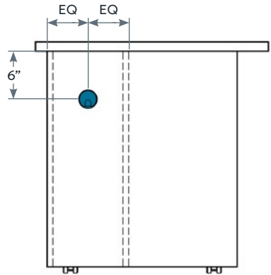
Grommet on Connector Table
