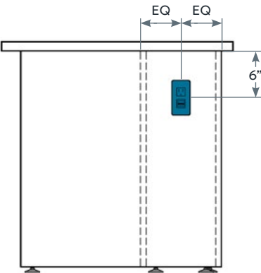
Carver Power on "C" Shape Table
