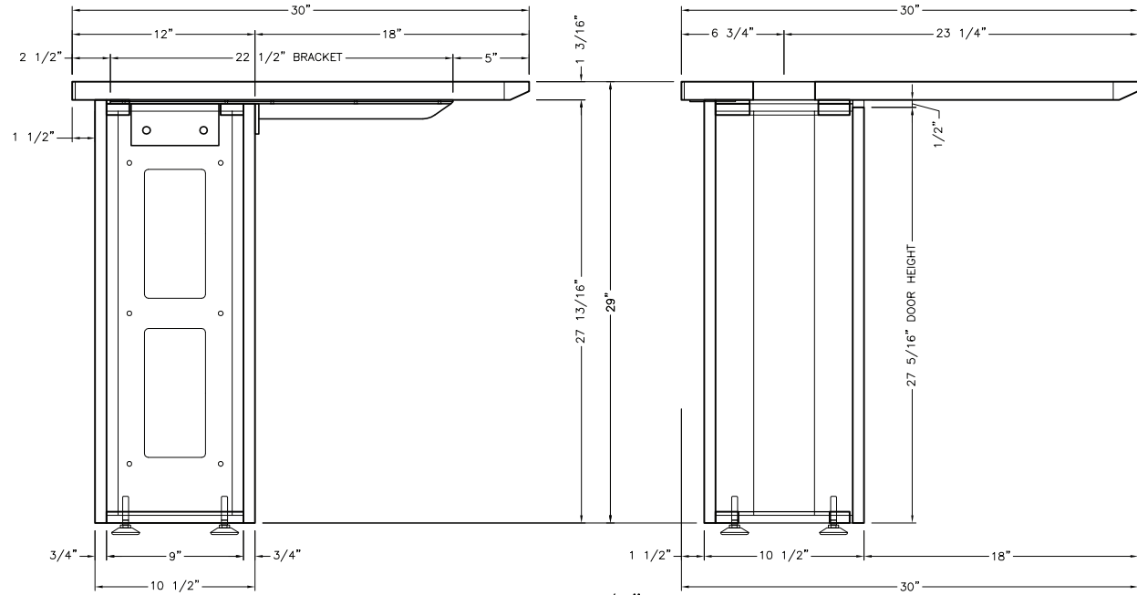
CROSS SECTIONS @ STD. 10-1/2"TH. WALL BASES
