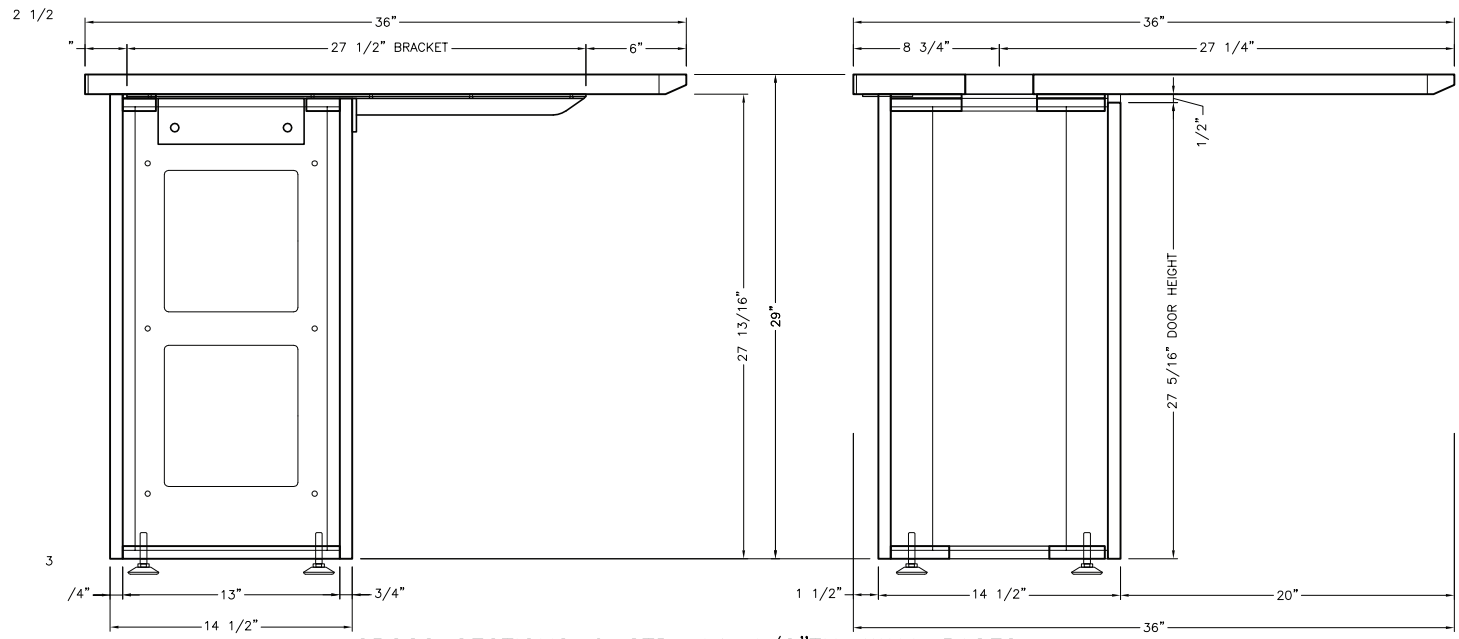
CROSS SECTIONS @ STD. 14-1/2"TH. WALL BASES
